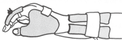
3. 手関節駆動型把持装具 (RIC 型)
